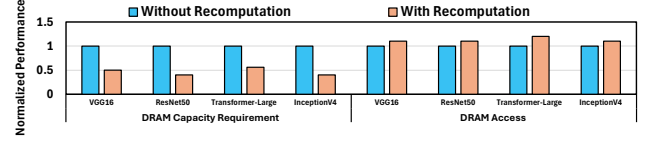
Figure 13: With recomputation enabled, Crane largely reduces DRAM capacity requirement with minor overhead (Batch size = 64).
